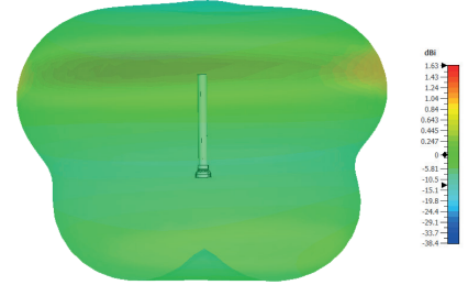
3D Plot Top Element (700MHz)
