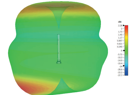
3D Plot Top Element (2000MHz)
