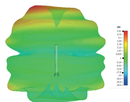
3D Plot Bottom Element (3600MHz)
