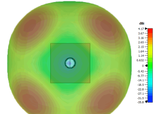
Typical 3D Pattern LTE Elements Top 1800MHz
