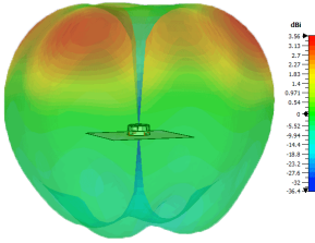
Typical 3D Pattern LTE Elements Side 800MHz
