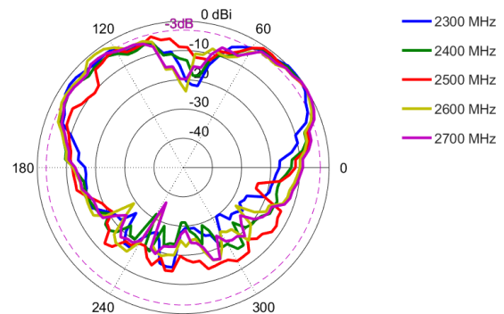
Azimuth: 2300 - 2700 MHz
