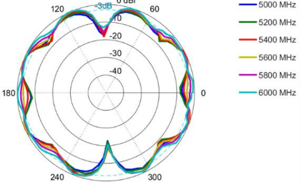
Elevation: 5000 – 6000 MHz
