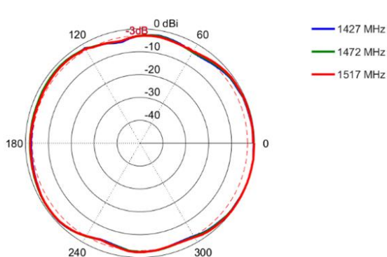
Azimuth: 1427 – 1517 MHz
