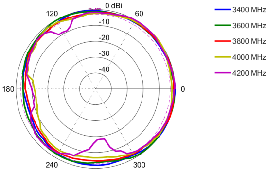
Azimuth: 3400 – 4200 MHz
