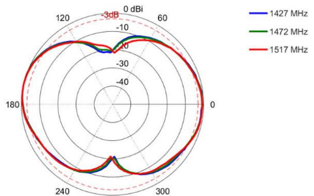
Elevation: 1427 – 1517 MHz
