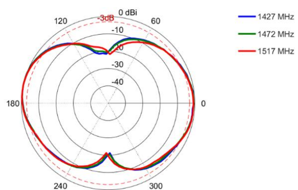
Elevation: 1427 – 1517 MHz
